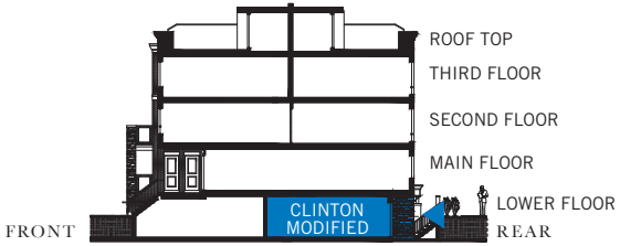
Typical Cross Section – Location Specific Buildings 1, 2, 3 + 5 only
