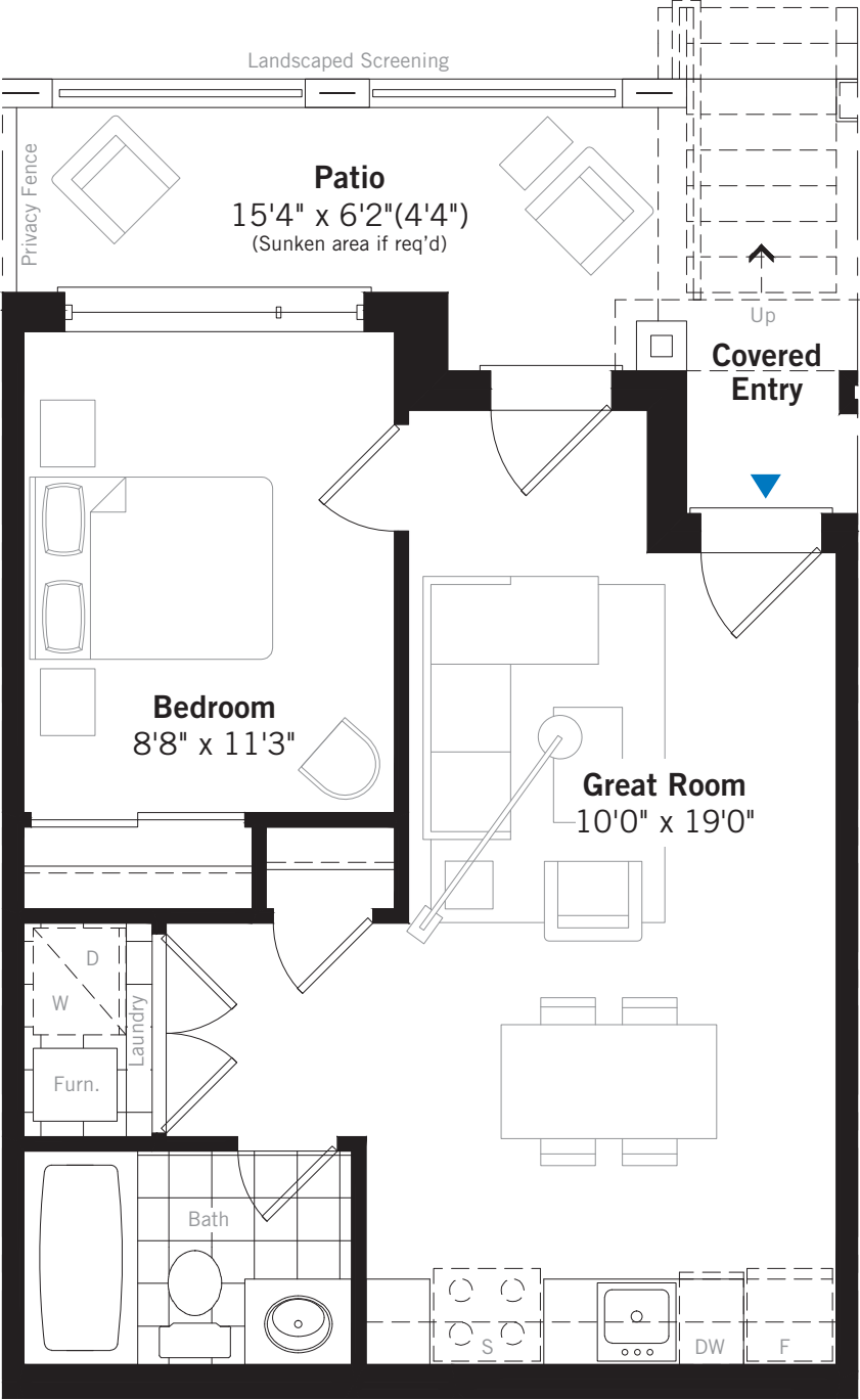
Typical Lower Floor Plan – One Bedroom Interior Condition – Rear
